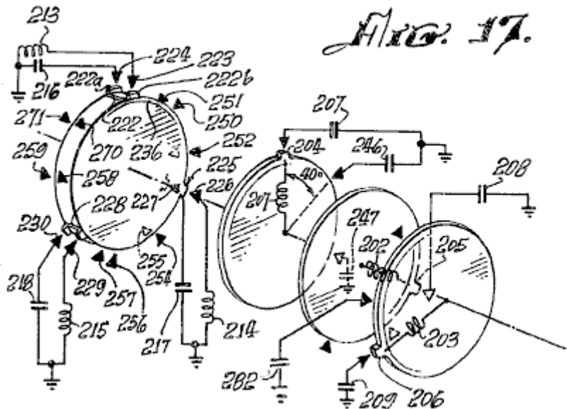
Fig.17 is a schematic diagram showing co-operating mechanical and electrical features of the programmer portion of the invention.
