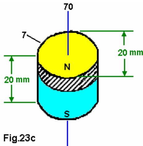
Fig.23c shows a preferred embodiment of a magnet 7 of rotor 1 . The magnet 7 is cylindrical with the magnetic dipole axis 70 coinciding with the longitudinal axis of the cylinder. The cylinder has a height of 20 mm and a diameter of 20 mm.
